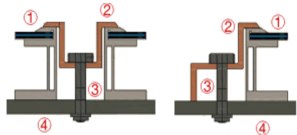
①frame ②clip ③ M8 bolt ④mounting rail
