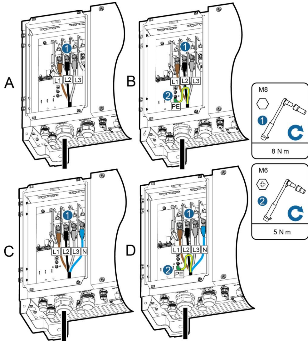
Abbildung 5-14 SUN2000-29.9KTL/33KTL-A/36KTL
